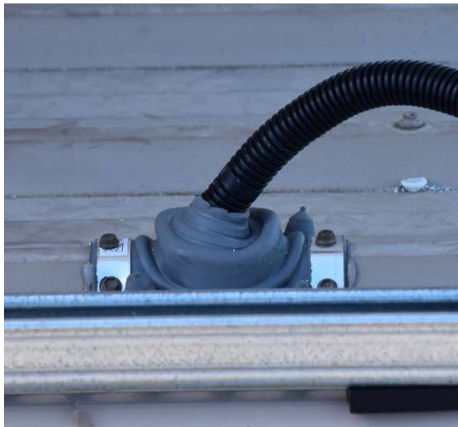
Figure 17: A collar flashing on a metal roof
