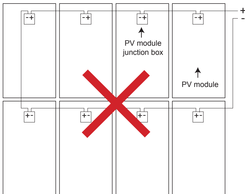
Figure 12: Example of wiring that will cause conductive loops and not to be done.
